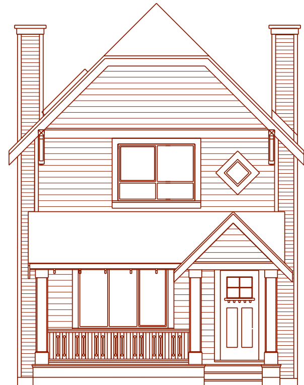
FRONT ELEVATION (MIRRORED)
